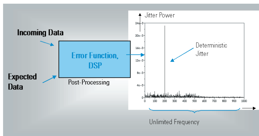
Figure 20: Jitter Decomposition by Spectrum Analysis
