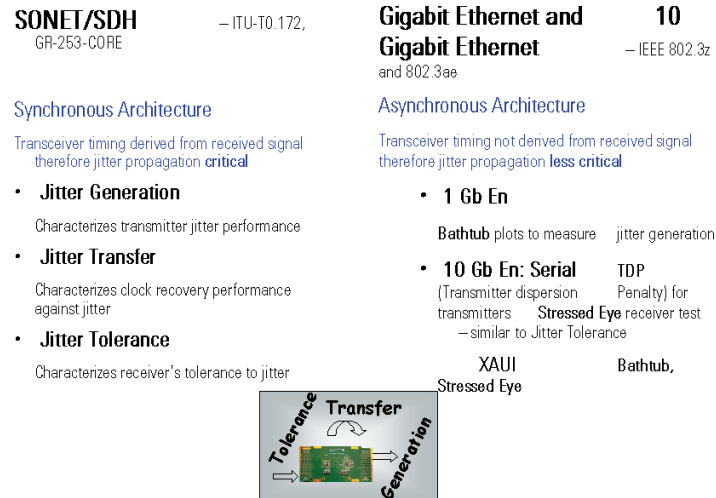
Figure 12: Jitter: The standards
