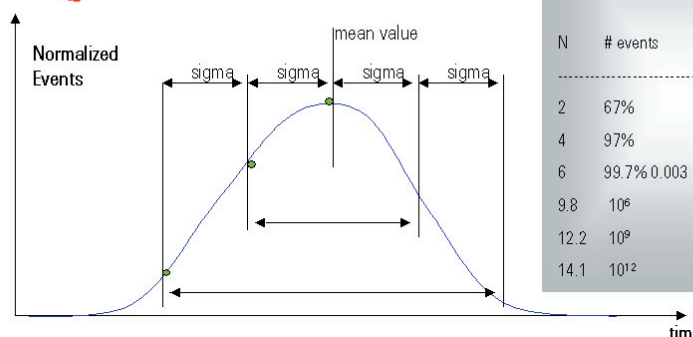
Figure 6: Random Jitter: The Gaussian Distribution
