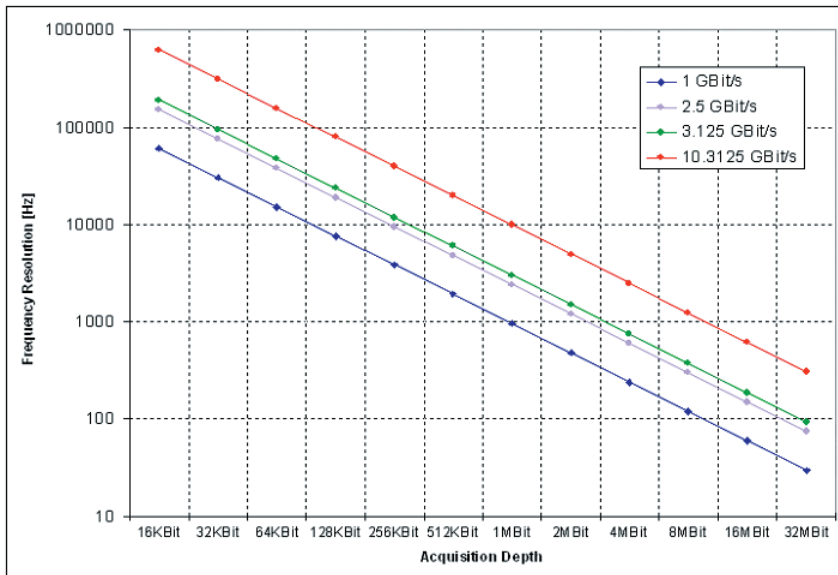
Figure 32: Frequency Resolution vs. Data
