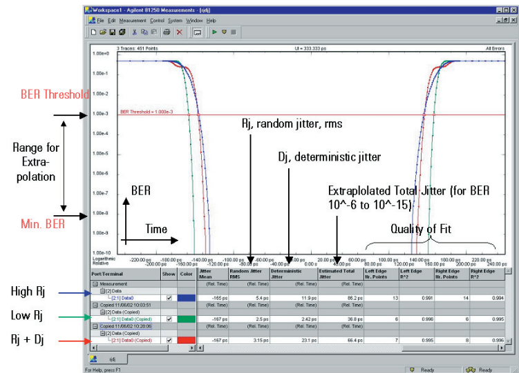
Figure 17: Serial BERT Bath Tub with RJ / DJ
