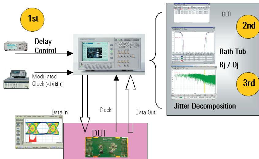
Figure 15: N4900 Serial BERT Jitter Capabilities
