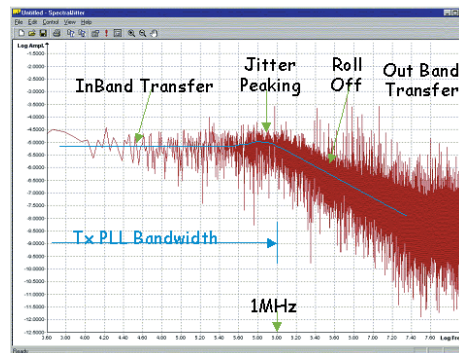
Figure 23: What Serial BERT's Jitter Decomposition is good for (2)
