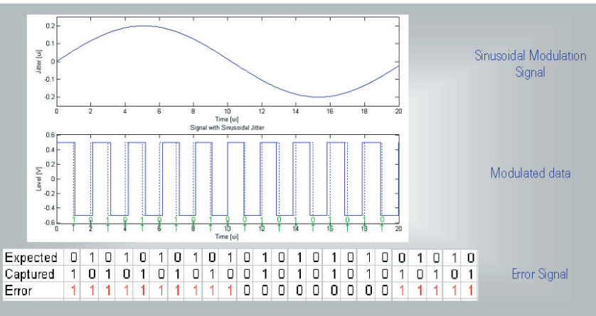
Figure 25: Basics of Method (2): Error Density Variation
