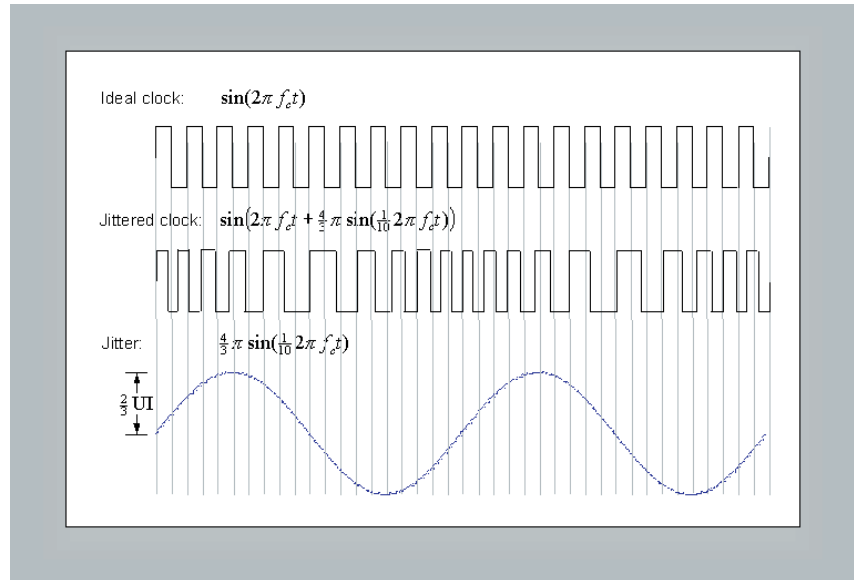
Figure 8: Periodic Jitter
