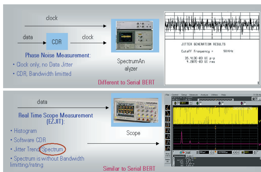
Figure 21: Existing Spectral Jitter Solutions
