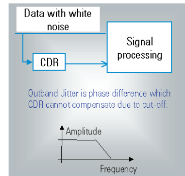
Figure 23: What Serial BERT's Jitter Decomposition is good for (2)
