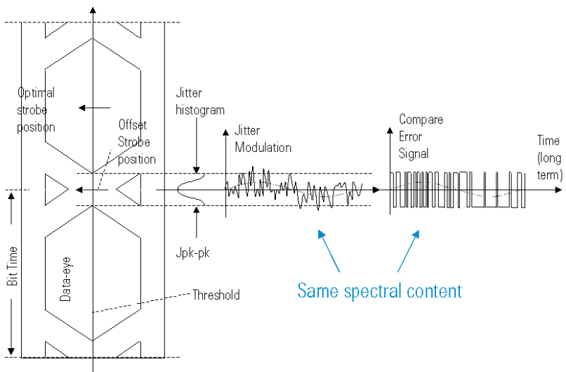
Figure 26: Basics of Method (3): The Noise is important
