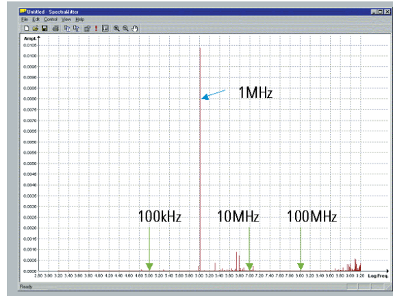
Figure 22: What Serial BERT's Jitter Decomposition is good for (1)
