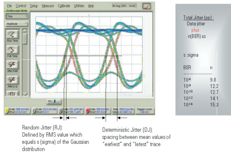
Figure 4: A real signal
