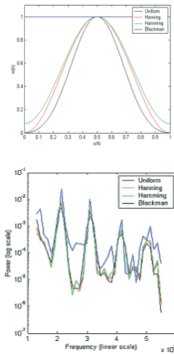
Figure 31: FFT Windowing
