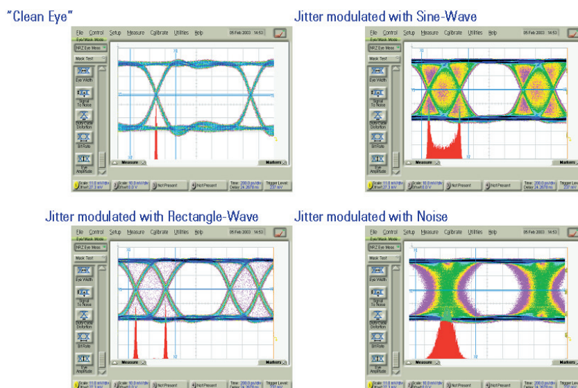
Figure 15: N4900 Serial BERT Jitter Capabilities
