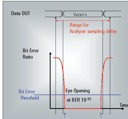
Figure 11: BERT Scan
