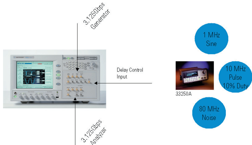
Figure 28: Simple Loop-back Measurements with help of Generator's Delay Control
