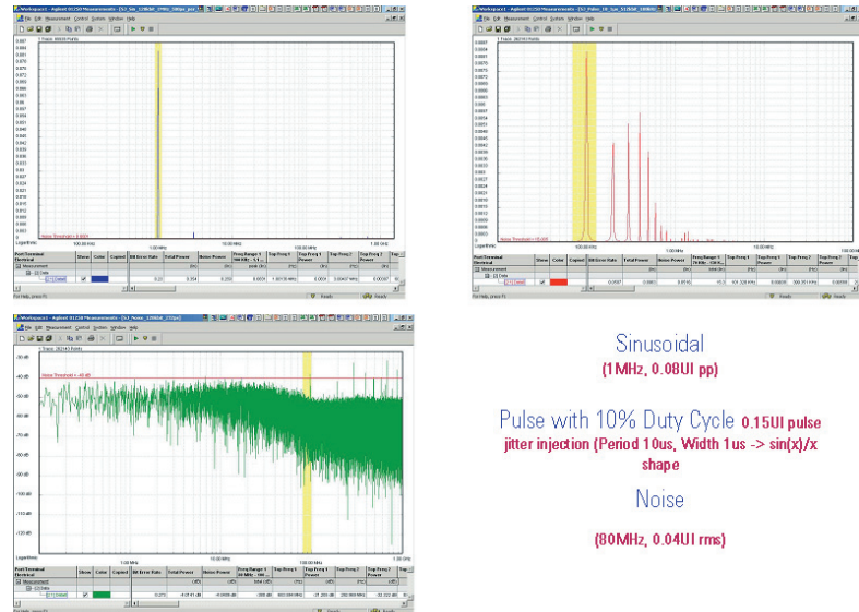
Figure 29: Jitter Decomposition Examples
