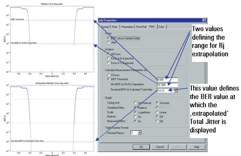
Figure 18: Bath Tub Properties for RJ / DJ
