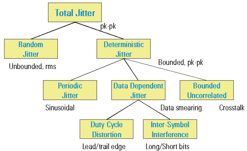
Figure 5: Jitter Component Segmentation
