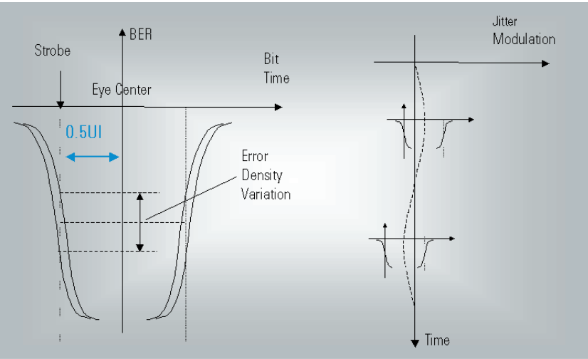
Figure 24: Basics of Method (1): Modulated Signal at Comparator
