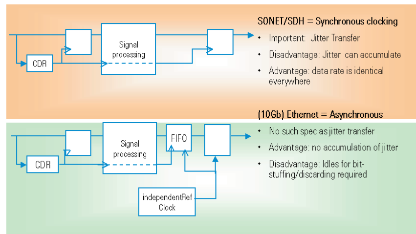
Figure 13: The difference in clocking of SONET/SDH and Ethernet
